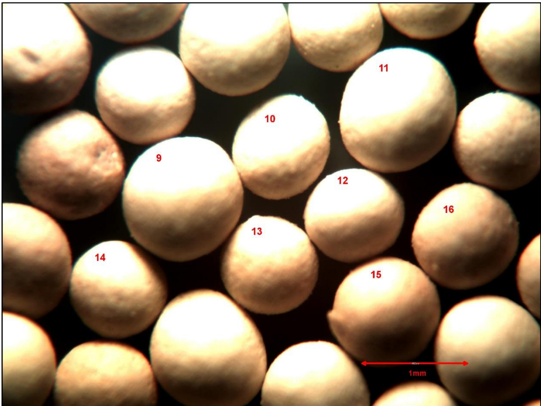
Proppant Sample - LWP (16/30)
