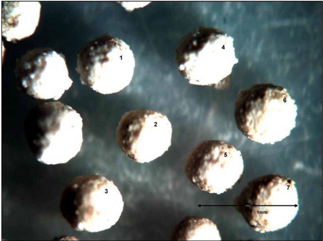
Proppant Sample - LWP 30/50 Yuanqu
